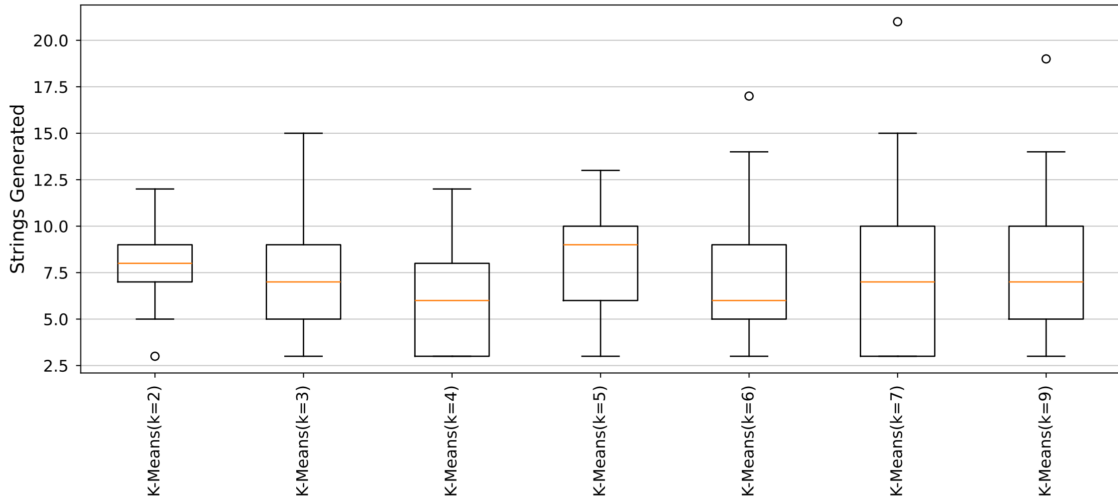
YARA Rules Strings Generated Distribution (Cluster14_Size9 dataset)
